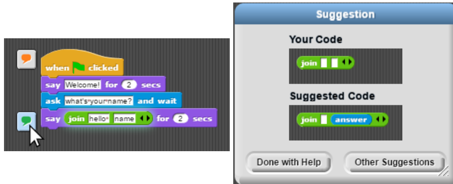
Fig. 1. A student’s code is annotated with hint buttons (left). Upon clicking a button, a hint window suggests a change to the student’s code (right).
